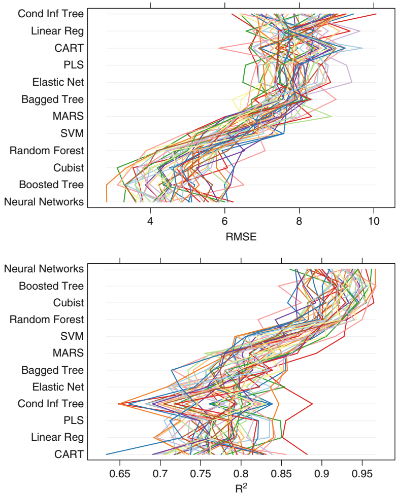
Fig. 10.2: Parallel coordinate plots for the cross-validated RMSE and R^2 across different models. Each line represents the results for a common cross-validation holdout set
