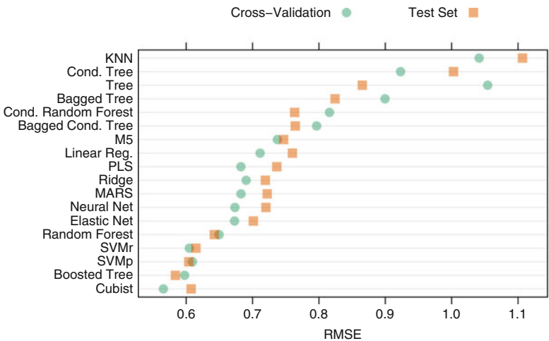
Fig. 9.2: A plot of the RMSE solubility models estimated by 10-fold cross-validation and the test set
