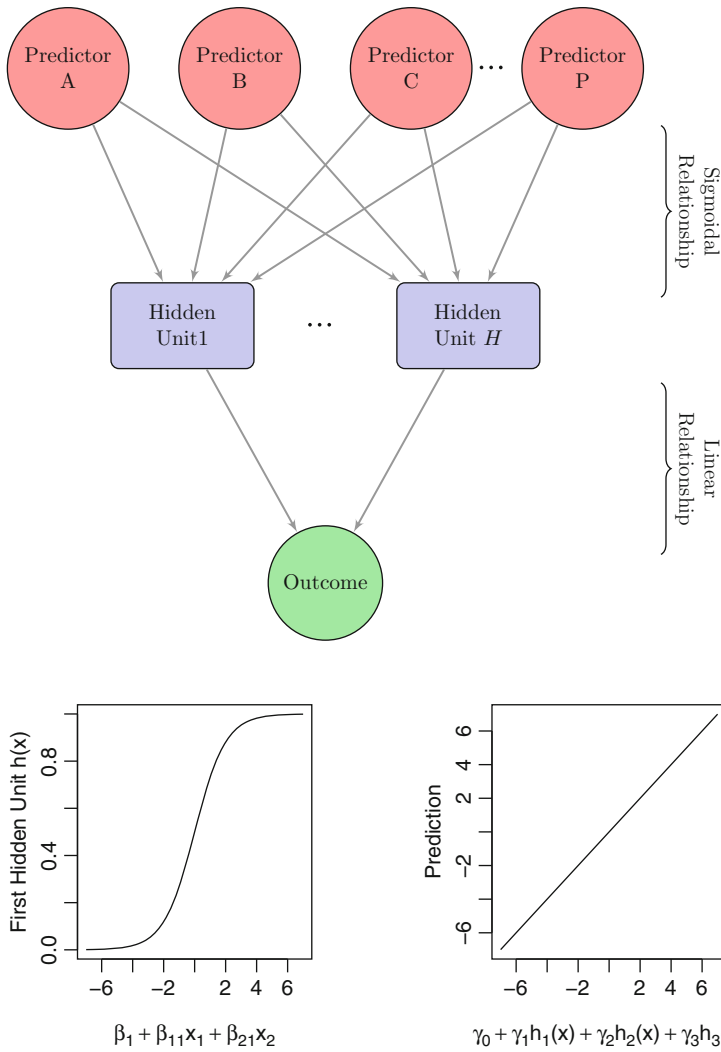
Fig. 7.1: A diagram of a neural network with a single hidden layer. The hidden units are linear combinations of the predictors that have been transformed by a sigmoidal function. The output is modeled by a linear combination of the hidden units
